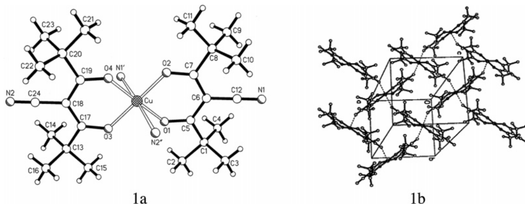
Figure 1. Single-crystal structure, 1a , and unit cell packing diagram, 1b , of \text{Cu}(\text{CNdpm})_2 adapted from ref 9. The immediate coordination geometry about \text{Cu}(\text{II}) is a tetragonally distorted octahedron exhibiting four short \text{Cu}-\text{O} equatorial bonds and 2 trans axial \text{Cu}-\text{N} bonds from adjacent molecules.
